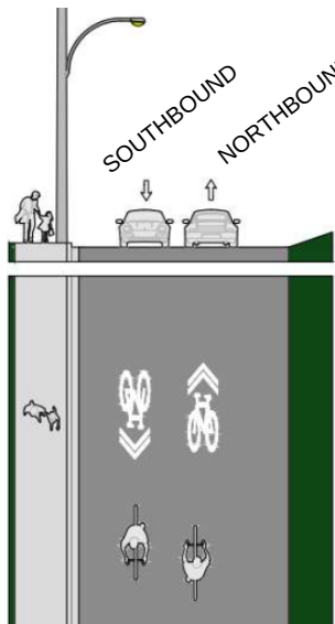
Neighbourhood Bikeway (two-way vehicle traffic)
