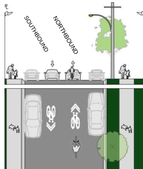
Neighbourhood Bikeway (two-way vehicle traffic)
